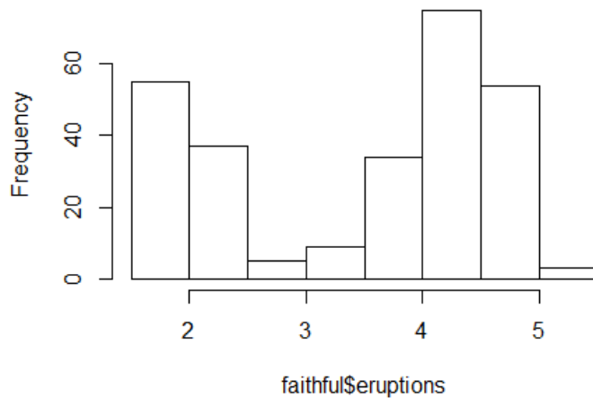
Histogram of faithful$eruptions
