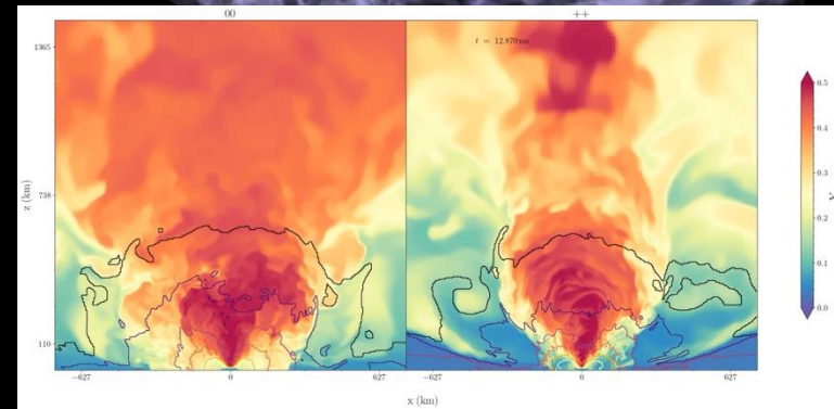
The effect of BNS spins on Y_e Allen Wen, AST GRA and FINESST
