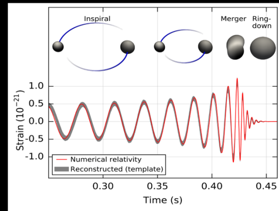
NR waveform modeling GW150914
