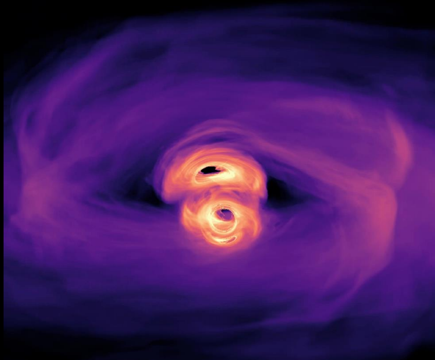
Intensity of X-rays (log scale) multiple-angle video in time, optically thin case
