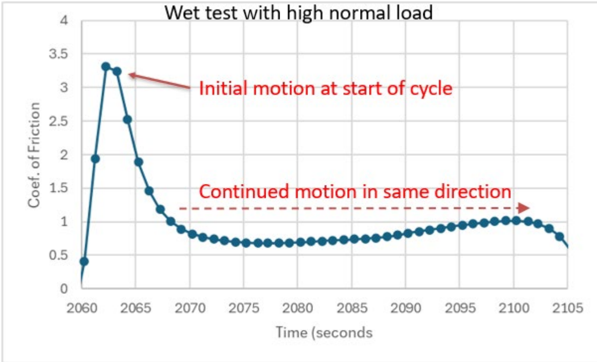
Figure 38. Characteristic COF Pattern: Wet Wood Crosstie.
