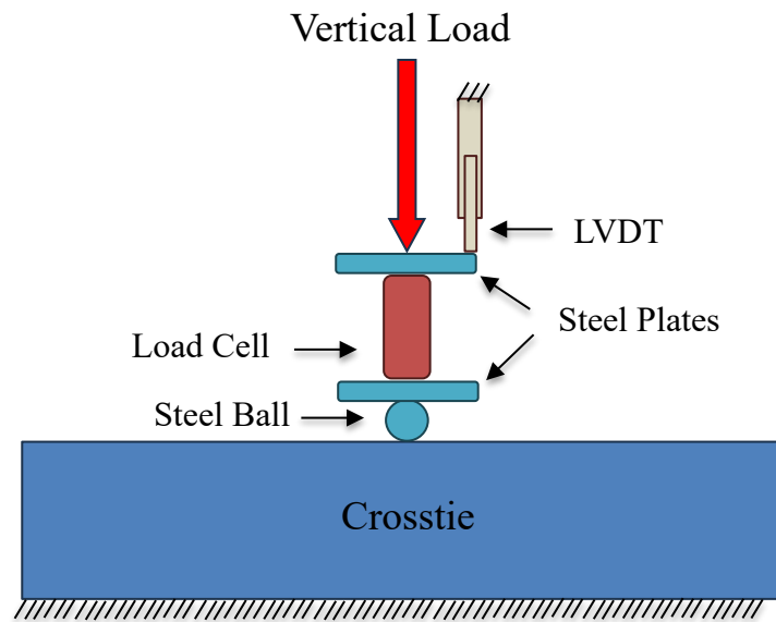
Figure 11. Schematic of Indentation Test.
