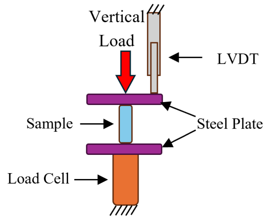
Figure 5. Schematic of Compression Test.
