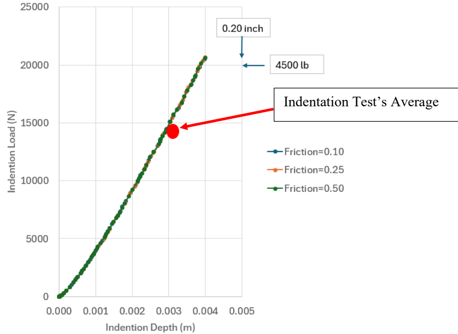
Figure 24. Axisymmetric Results: HDPE, 36.5 mm Ball.
