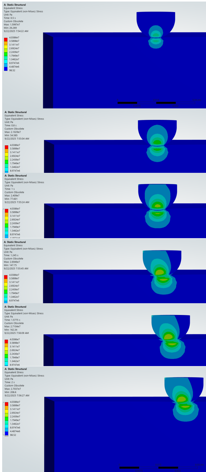
Figure 27. Half-symmetry Model of Indenter: Example Results.
