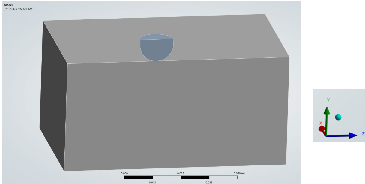
Figure 25. Half-symmetry Model of Indenter.
