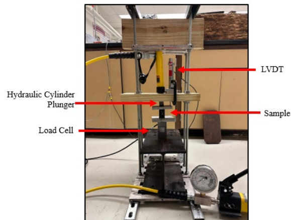
Figure 6. Compression Test Frame with Sample.
