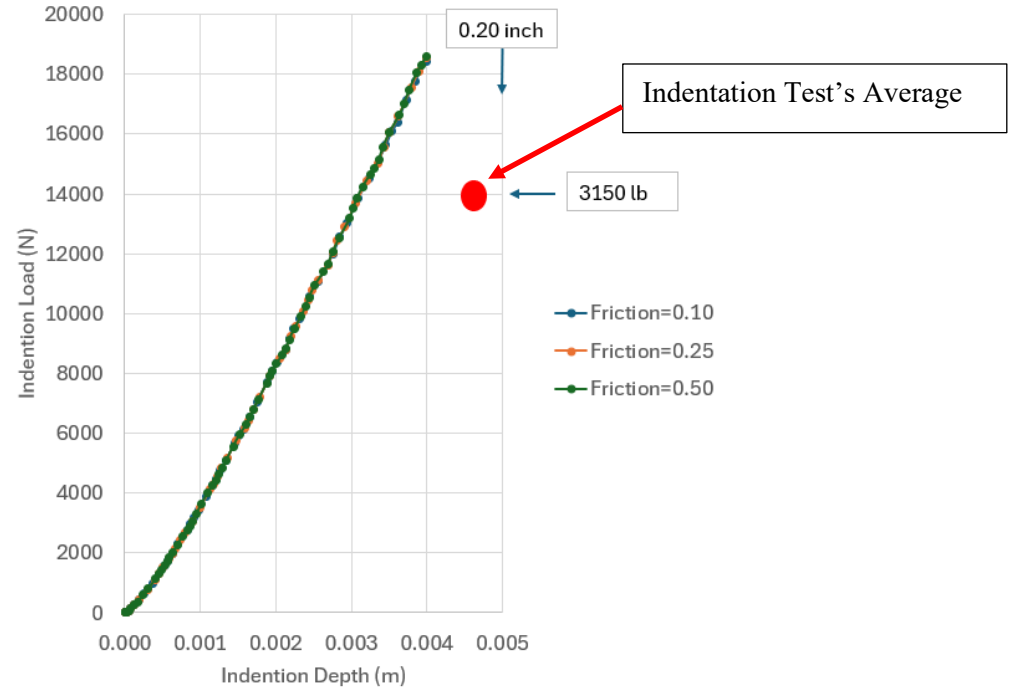
Figure 20. Axisymmetric Results: Dry Wood, 36.5 mm Ball.
