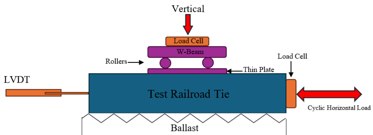
Figure 33. Friction Test Configuration.
