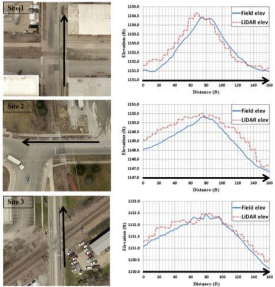
Figure 4.1 Comparison of vertical elevation profiles for LiDAR and field-measured data
