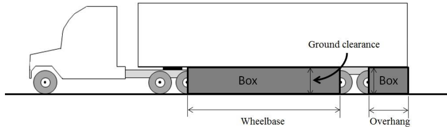
Figure 4.2 Semi-trailer with imaginary box under the trailer
