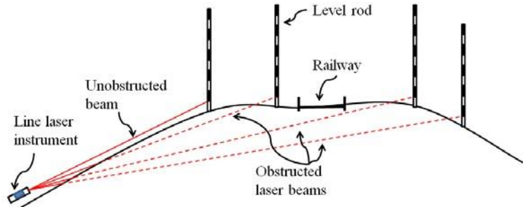
Figure 4.4 Illustration of the field validation of GIS-derived results
