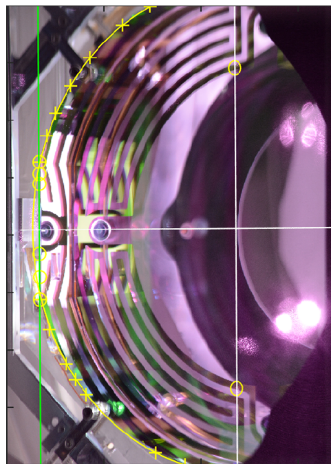
FIG. 11. Image of an end test mass from a Pcal beam localization camera system. The right side is occluded by the stray-light baffling. The mirrors have flats on the sides for attachment of the suspension fibers. These flats are oriented vertically and are used to determine the azimuthal orientation of the images. The well-defined angle of view along with the dimensions of the mirror enable the determination of the beam positions on the mirror surface by identifying points on the edge of the optic (yellow crosses) and fitting the appropriate ellipse to the points. The system is designed to determine the optimal positions of the beams on the mirror surface (yellow circles above and below center) with millimeter accuracy.
